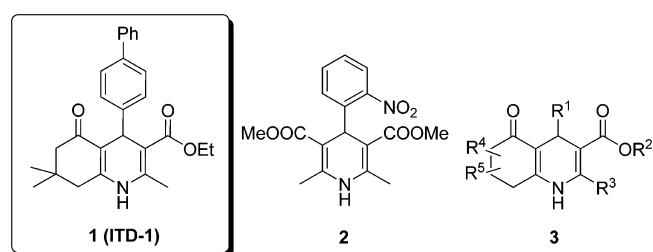
Figure 1. Chemical structures of 1,4-DHPs: 1 = cardiogenic “hit” from a mESC high-content screen, 2 = calcium channel blocker nifedipine, 3 = b -annulated 1,4-DHPs with weak calcium modulating activity reported in the literature. 4–6
