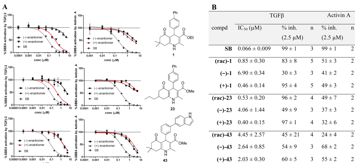
Figure 4. Effect of stereochemistry of 1,4-DHPs 1 , 23 , and 43 on TGFβ and Activin A inhibition. (A) Dose–response profiles of (+)- and (–)-enantiomers for TGFβ and Activin A inhibition. (B) Table of TGFβ and Activin A inhibition parameters, data represent means ± SD of n = 2–5 independent experiments. SB = SB-431542, a literature-reported TGFβ inhibitor (Alk-4/5/7 inhibitor). 21
