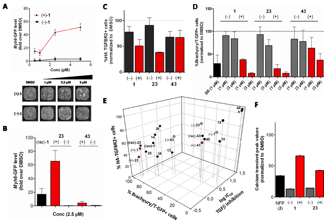
Figure 5. Characterization of 1,4-DHP enantiomers in secondary functional assays. (A) Cardiogenesis in Myh6 -GFP mESC cells: lower panel illustrates representative whole-well images of mESCs on day 10 of differentiation after treatment with (+)- or (-)-enantiomers of 1 compared to media and DMSO controls, upper panel shows the corresponding plot after image analysis (mean \pm SD, normalized to DMSO = 1-fold). (B) Cardiogenesis in Myh6 -GFP mESC cells: (+)- or (-)-enantiomers of 23 and 43 compared to (rac)- 1 at 2.5 \mu M (mean \pm SD, normalized to DMSO = 1-fold). (C) TGFBR2 degradation (down-regulation) in HEK-293T cells: % HA-tagged TGFBR2 positive cells after treatment with (+)- or (-)-enantiomers of 1 , 23 , or 43 at 3 \mu M doses (mean \pm SD, normalized to DMSO = 100%). (D) Mesoderm inhibition with J1 Brachyury/T-GFP mESC cells: % T-GFP positive cells after treatment with (+)- or (-)-enantiomers of 1 , 23 , or 43 at 1 and 3 \mu M, normalized to DMSO = 100%. (E) 3D correlation plot: x -axis, TGF \beta /Smad inhibition values (log IC 50 ); y -axis, mesoderm inhibition with J1 Brachyury/T-GFP mESC cells at 3 \mu M 1,4-DHP doses (% Brachyury/T-GFP positive cells, normalized to DMSO = 100%); z -axis, TGFBR2 degradation values at 3 \mu M 1,4-DHP doses (% HA-TGFBR2 positive cells, normalized to DMSO = 100%). (F) Calcium transient peak values in HL-1 cells: comparison of Ca 2+ transient peak values (Fluo4 levels, average pixel intensity) in the presence of (+)- and (-)-enantiomers of 1 and 23 (mean \pm SEM).
