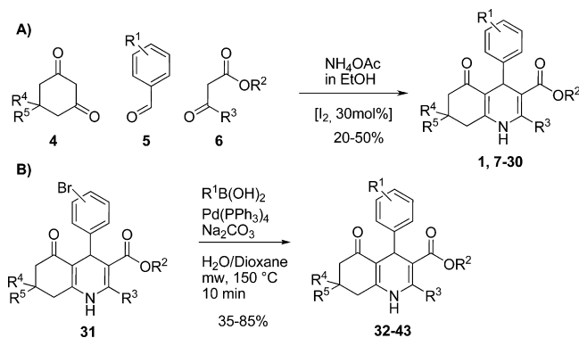
Scheme 1. Synthesis of Racemic 1,4-DHPs
